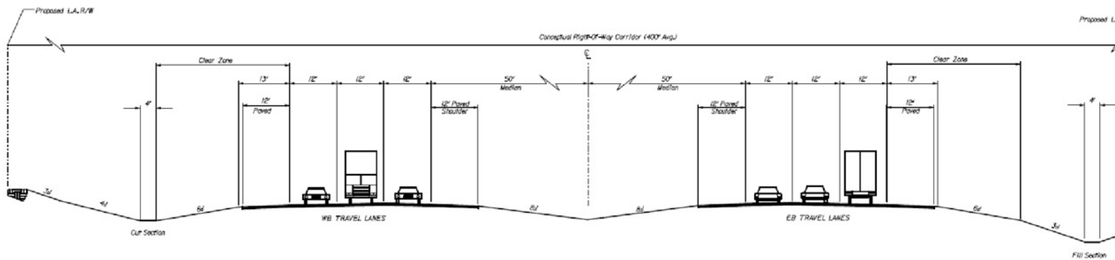
Figure 5.3 Typical Cross Section, 6-Lane Rural
