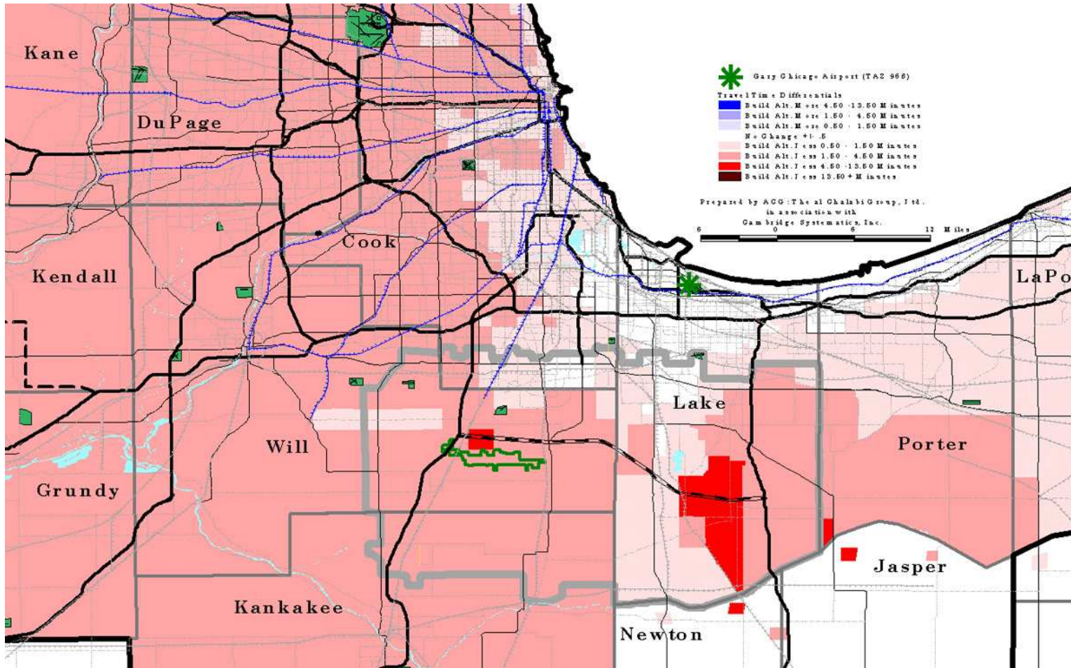
Figure 8.22 Travel Time Differentials to Gary Chicago Airport 2030 Hybrid Build Alternative (AC2) as Compared to 2030 No-Build Network
