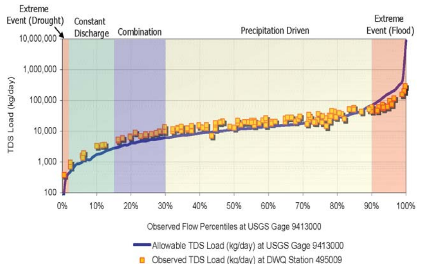
Figure 7-5. Example load duration curve.
