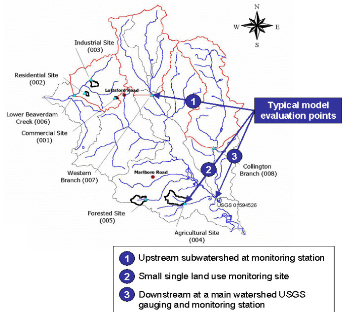
Figure 8-2. Typical model evaluation points.
